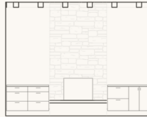
FIREPLACE ELEVATION
